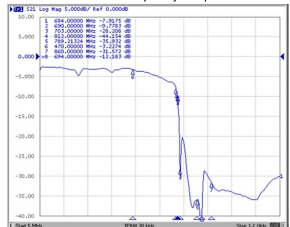
LTE Balun Frequency Response
