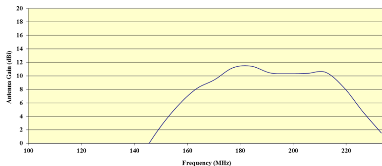
Antenna Gain (dBi) vs. Frequency (MHz)
