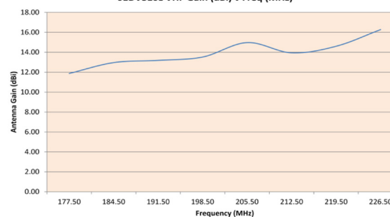
01DV310L VHF Gain (dBi) v Freq (MHz)
