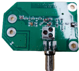
PCBA with 4G/5G rejection
