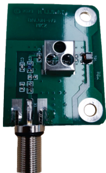
PCBA with 4G/5G rejection
