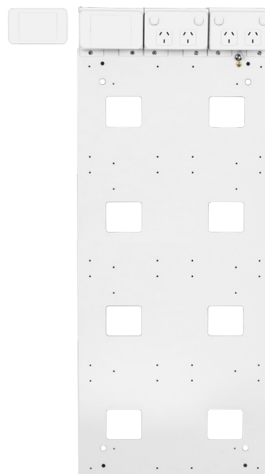
Gear Tray with 3x Mounting Blocks (2x Blank Plates & 2x Double GPO)
