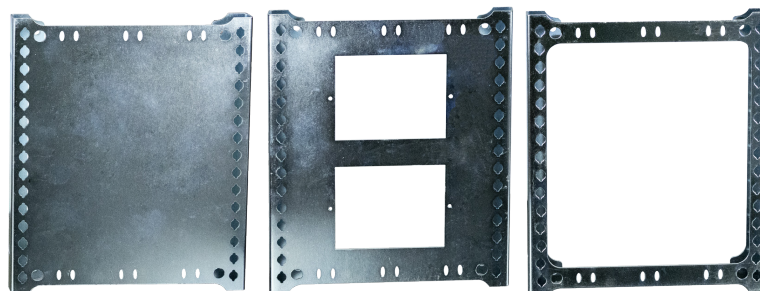
Gear Tray with 3x Mounting Blocks (2x Blank Plates & 2x Double GPO)
