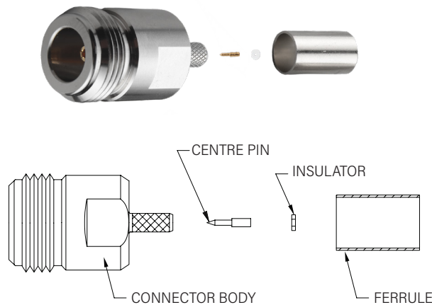
Connector Parts
