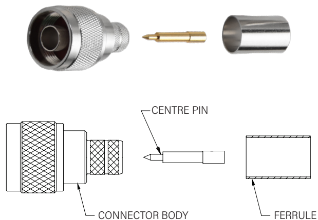
Connector Parts
