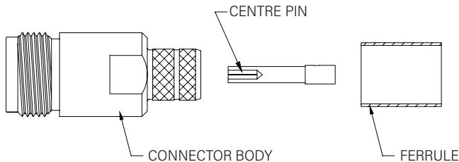
Connector Parts
