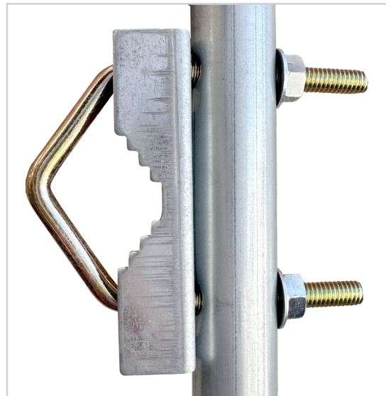
Close-up of U-Bolt & V-Block
